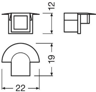
Slim Profile 12 mm height, 3 mm wings FX-QMS-G1-TU16H12W3-300 Order code 4052899448988
