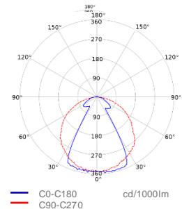
Profile without cover
