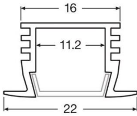
Slim Profile 12 mm height, 3 mm wings FX-QMS-G1-TU16H12W3-300 Order code 4052899448988
