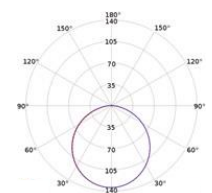
— C0-C180 cd/1000lm — C90-C270
