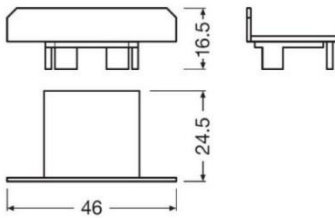
Plastic flat end cap FX-QMW-G1-EFGP-TU26H25W10 Order code 4052899450134
