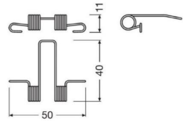
Mounting spring metal FX-QMW-G1-SRME-DIV1 Order code 4052899446786
