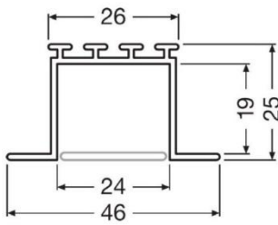
Wide Profile 25 mm height, 10 mm wings FX-QMW-G1-TU26H25W10-300 Order code 4052899448773
