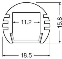
Slim Profile round FX-QMS-G1-TR19H16-300 Order code 4052899449008
