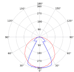
— C0-C180 — C90-C270 cd/1000lm
