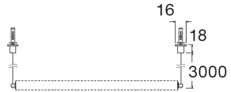
Pendant Kit FX-QMS-G1-TR19H16-PENDANTKIT Order code 4052899600034
