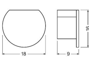
Plastic End cap FX-QMS-G1-EFGP-TR19H16 Order code 405289999985
