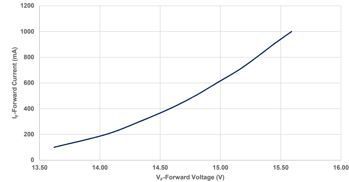
Figure 6: Typical forward current vs. forward voltage @ T_C = 25^{\circ}\text{C}
