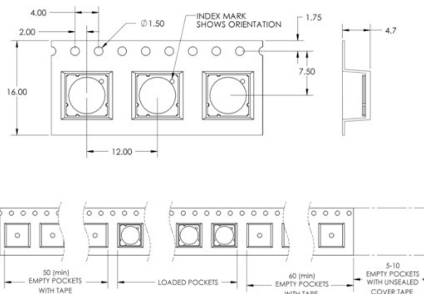
Figure 12: Emitter carrier tape specifications (mm)
