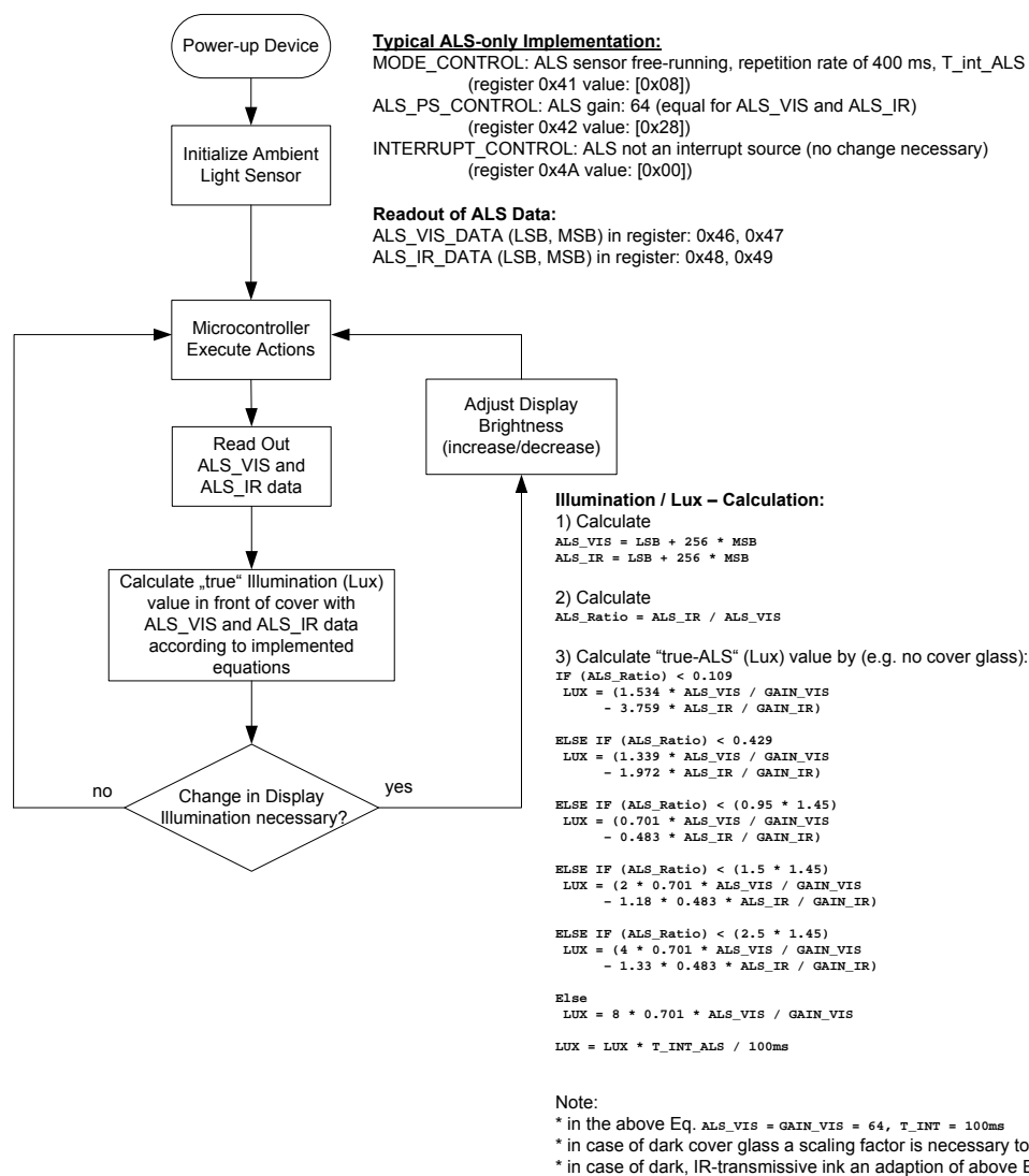
Fig. 23: Flowchart for a microcontroller based ambient light sensing example. After performing the ALS_IR/ALS_VIS ratio calculation the true illumination (lux) value can be directly calculated according to the Eqs. Please note that these Eqs. need to be adapted to the characteristic cover glass transmission properties (e.g. a simple gain factor to account for the attenuation if implemented behind a dark cover glass with flat transmission characteristics (visible to infrared range) or by adaption of the parameters if implemented behind dark, IR transmissive cover glasses). See Sec. 10.1 for more details.
