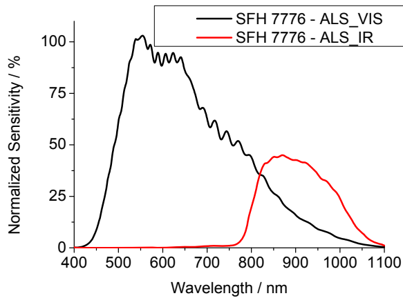
Fig. 3: Spectral sensitivity of the two ALS sensors of the SFH 7776 (ALS_VIS and ALS_IR have equal gain setting).
