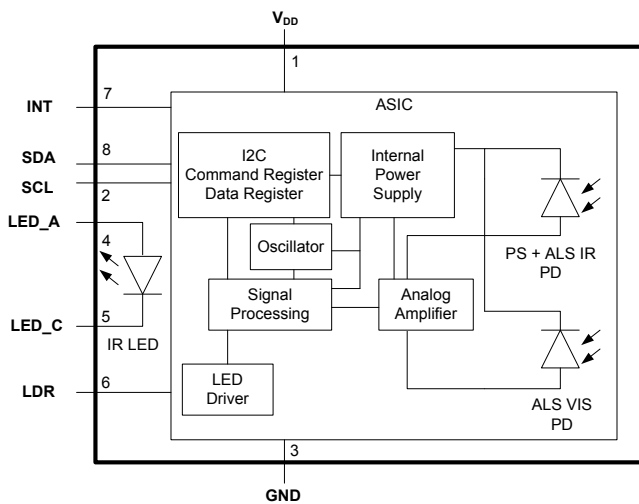
Fig. 2: SFH 7776 functional block diagram.
