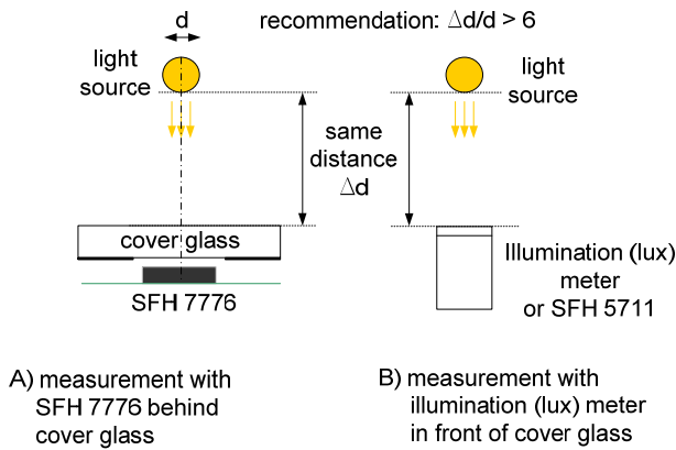
Fig. 16: Measurement setup for deriving the required equations to calculate the illumination (lux) value out of ALS_VIS, ALS_IR.
