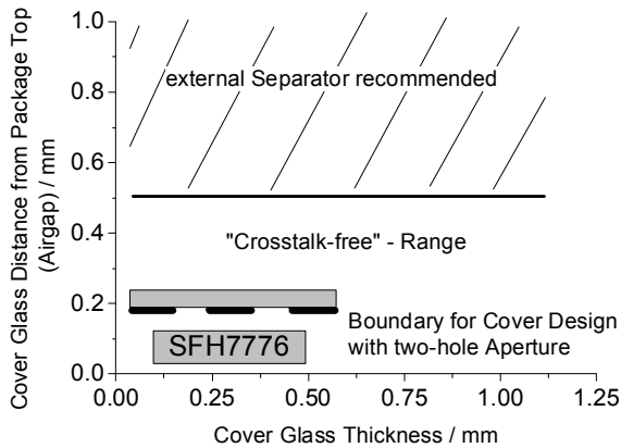
Fig. 12: Crosstalk-free range: Cover glass thickness vs. airgap. The device is "crosstalk-free" for e.g. 1.0 mm cover glass and an airgap of 0.5 mm. To achieve optimized performance a two-hole aperture design is recommended (see Fig. 13).
