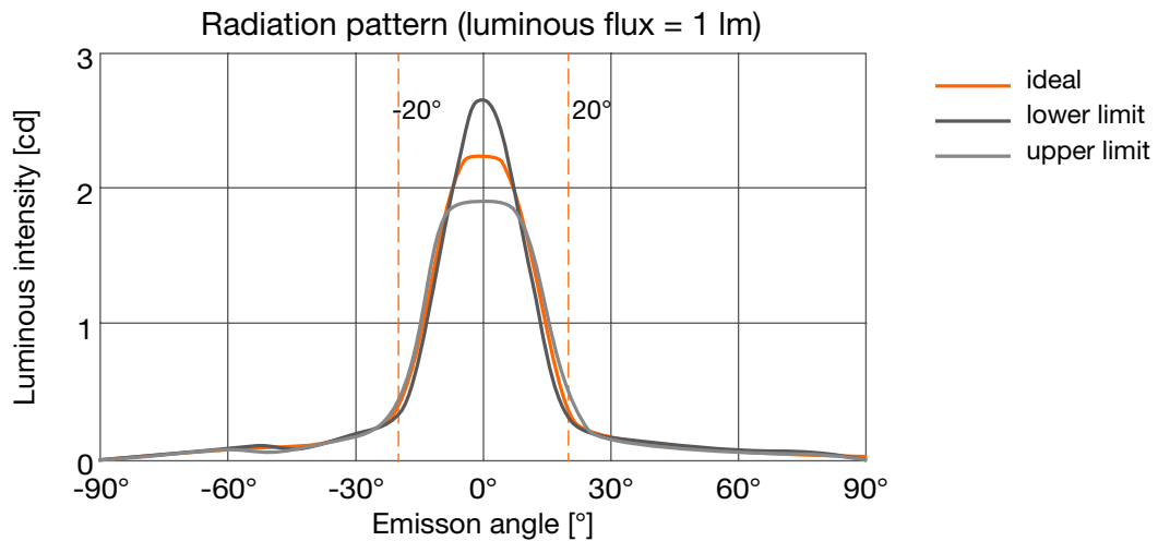
Figure 5: Emission characteristics
