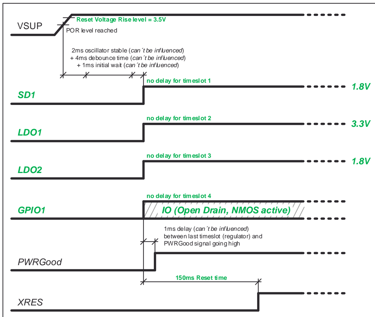
Figure 2: Startup digram for AS3701B-BWLM-02
