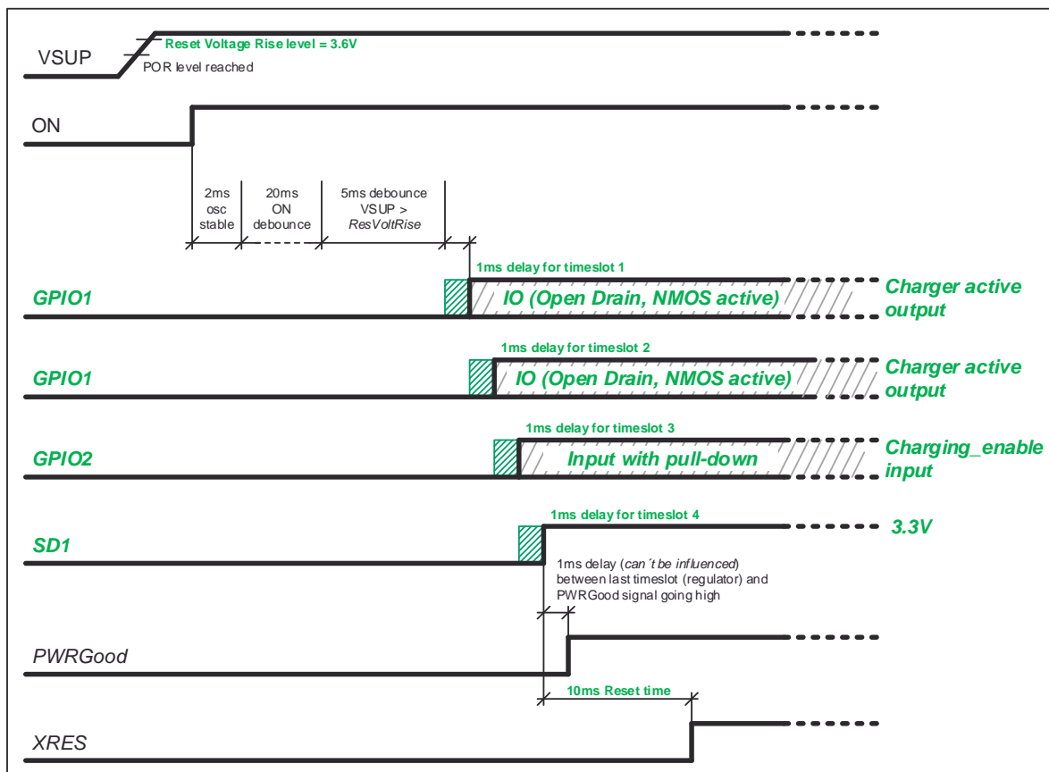
Figure 2: Startup digram for AS3701A-BWLM-50
