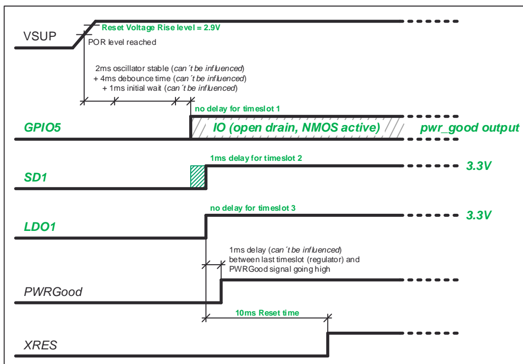
Figure 2: Startup digram for AS3701B-BWLM-68
